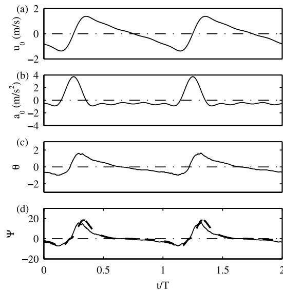
Figure 14. Sediment transport under saw-tooth wave of wave period T = 6.0 s. (a) Prescribed free-stream velocity, (b) free-stream acceleration, and (c) nondimensional bed shear stress. (d) Nondimensional sediment transport rate using calculated nondimensional bed shear stress and Meyer-Peter Müller formula (solid curve) and two-phase sheet flow model (dashed curve).
